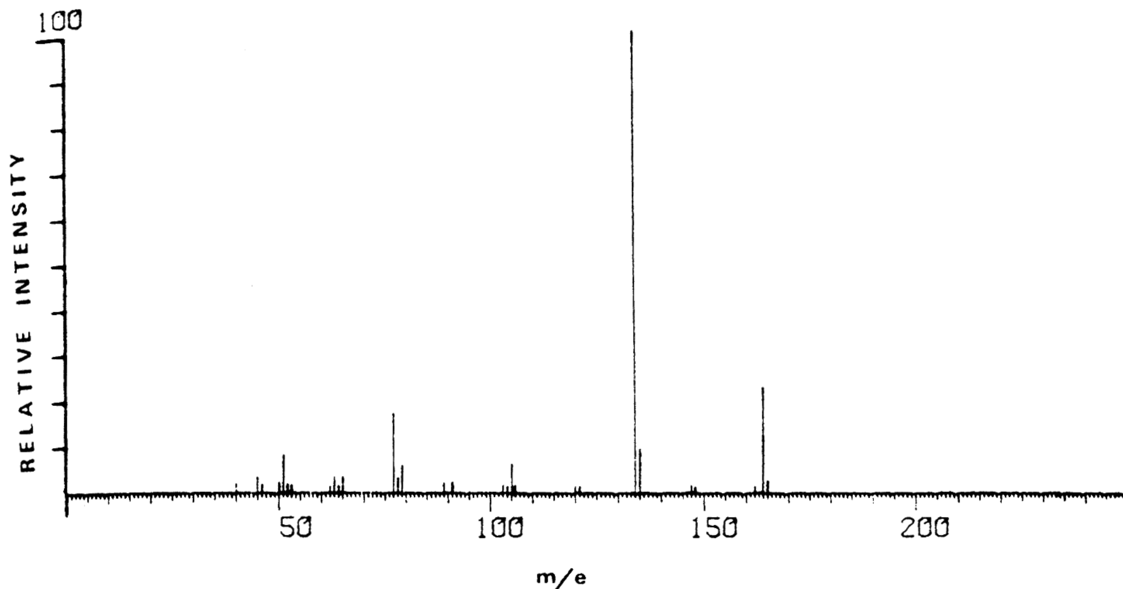
FIG. 19—Mass spectrum of 3,4-methylenedioxyphenylpropane.
