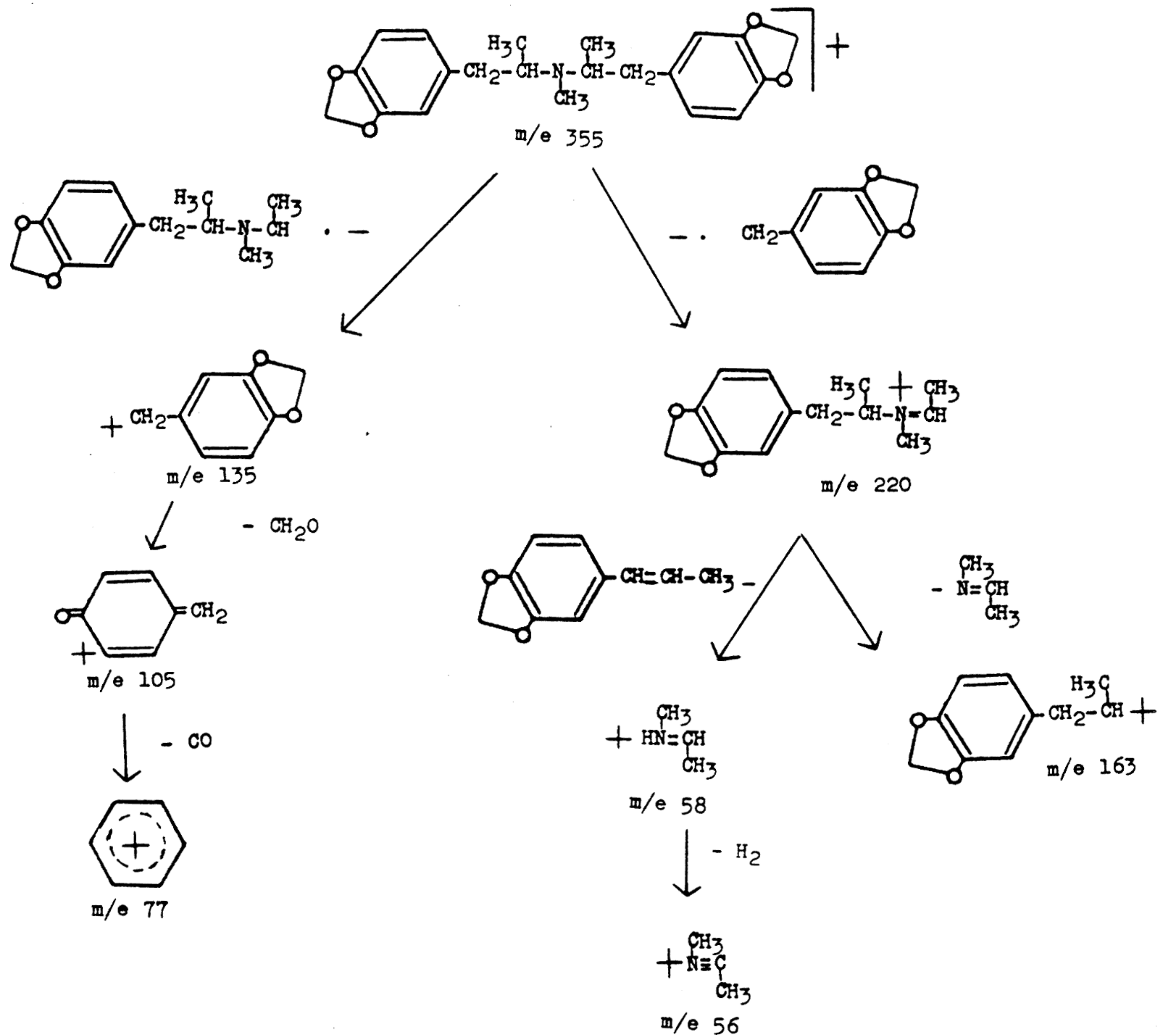
FIG. 12—Proposed fragmentation pattern of di[1-(3,4-methylenedioxyphenyl)-2-propyl]methylamine.
