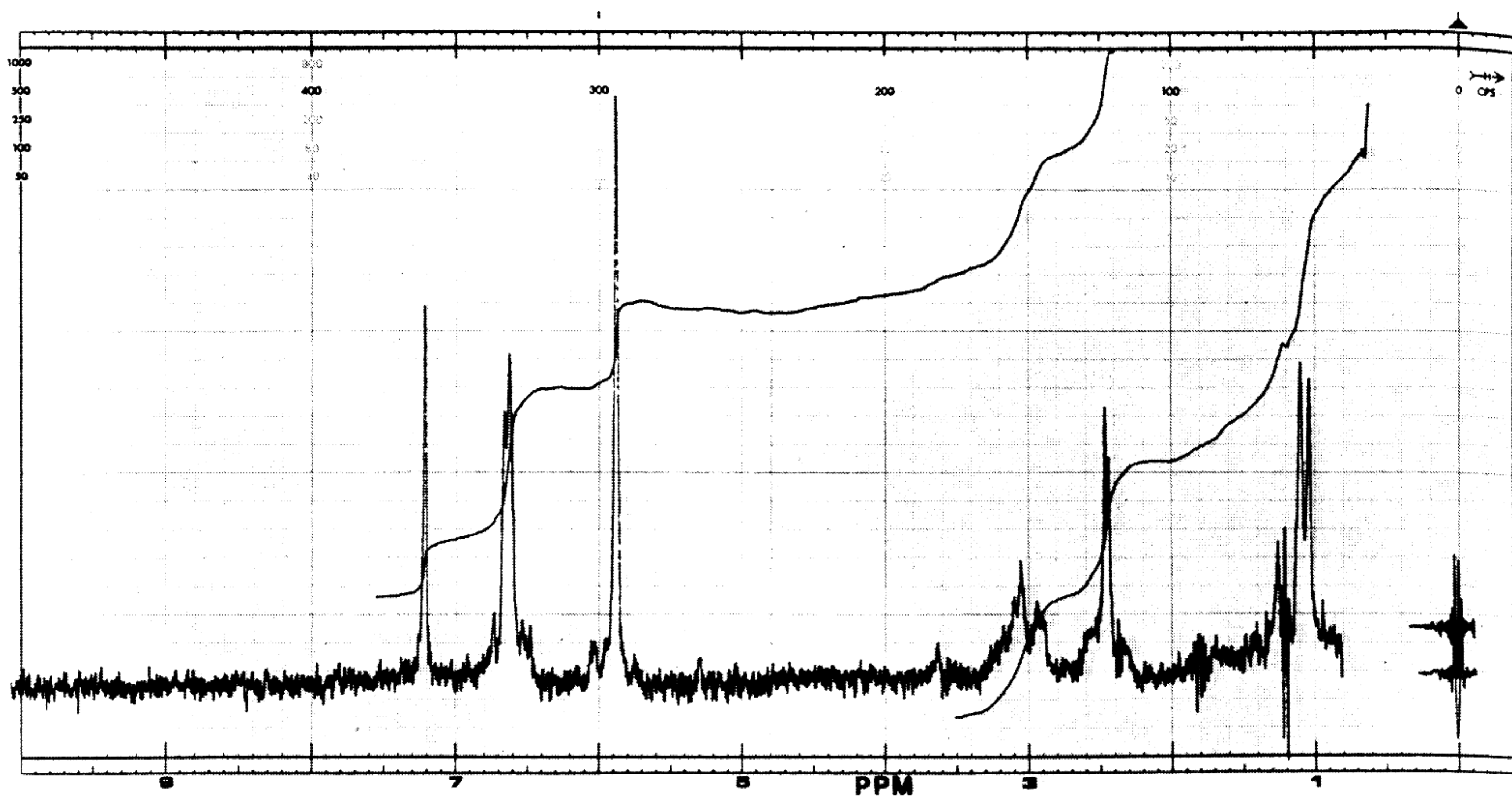
FIG. 13—NMR spectrum of di[1-(3,4-methylenedioxyphenyl)-2-propyl]methylamine.
