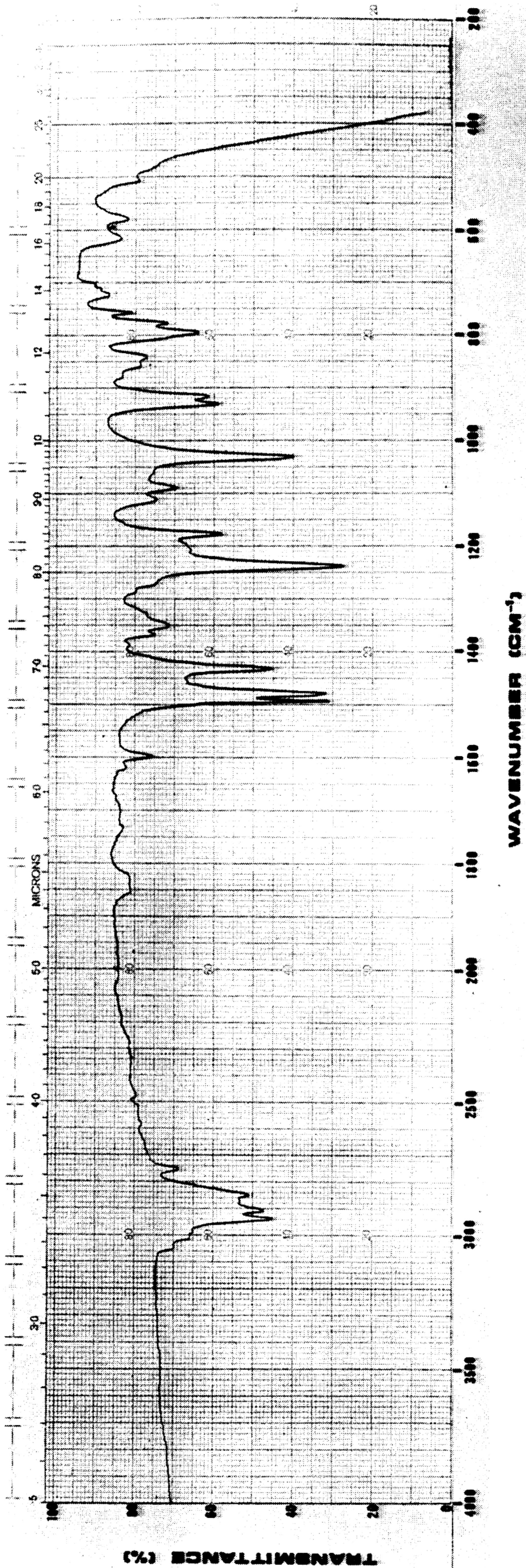
FIG. 18—IR spectrum of 3,4-methylenedioxyphenylpropane.
