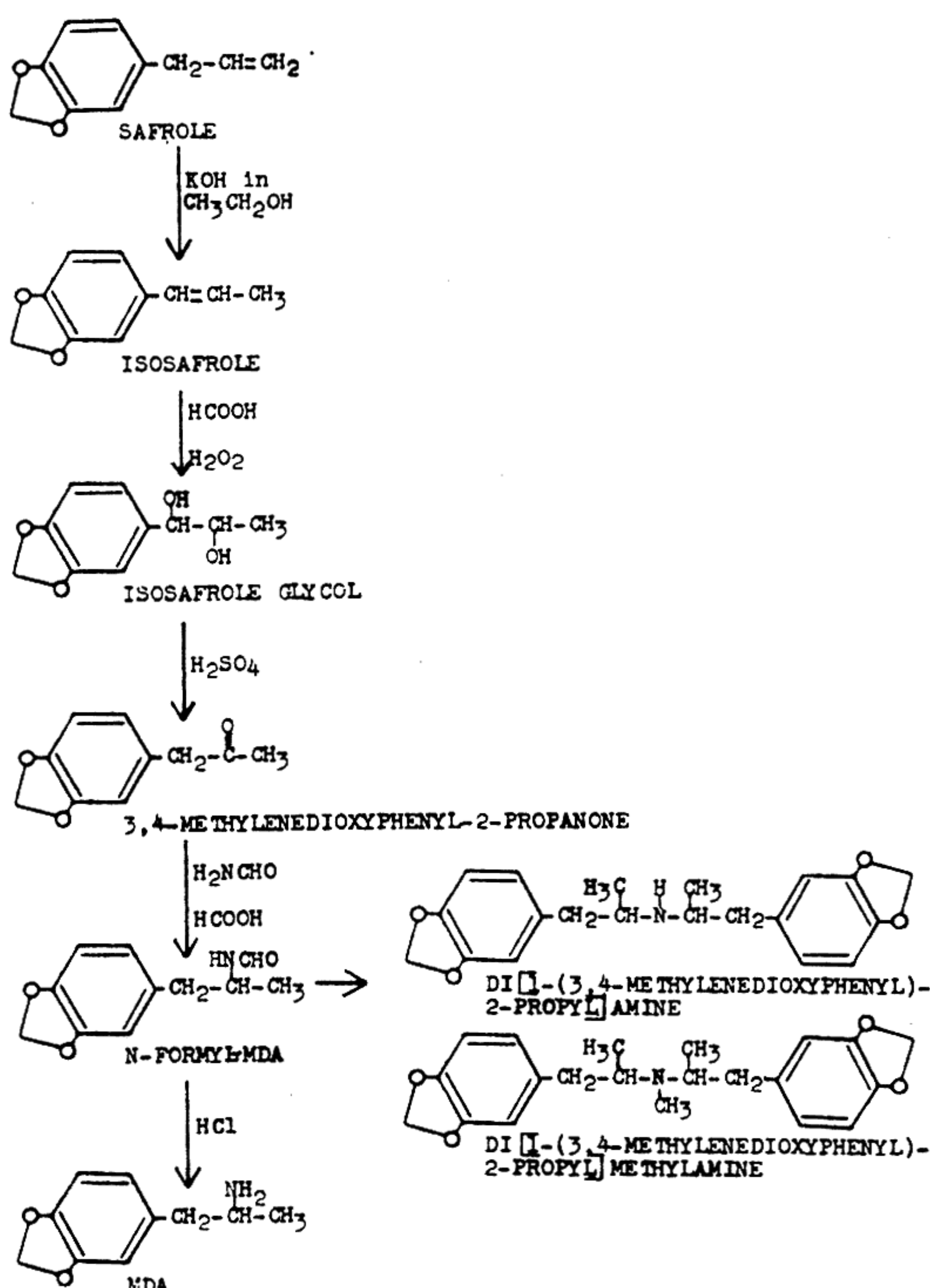
FIG. 1—Synthesis of MDA from safrole.
