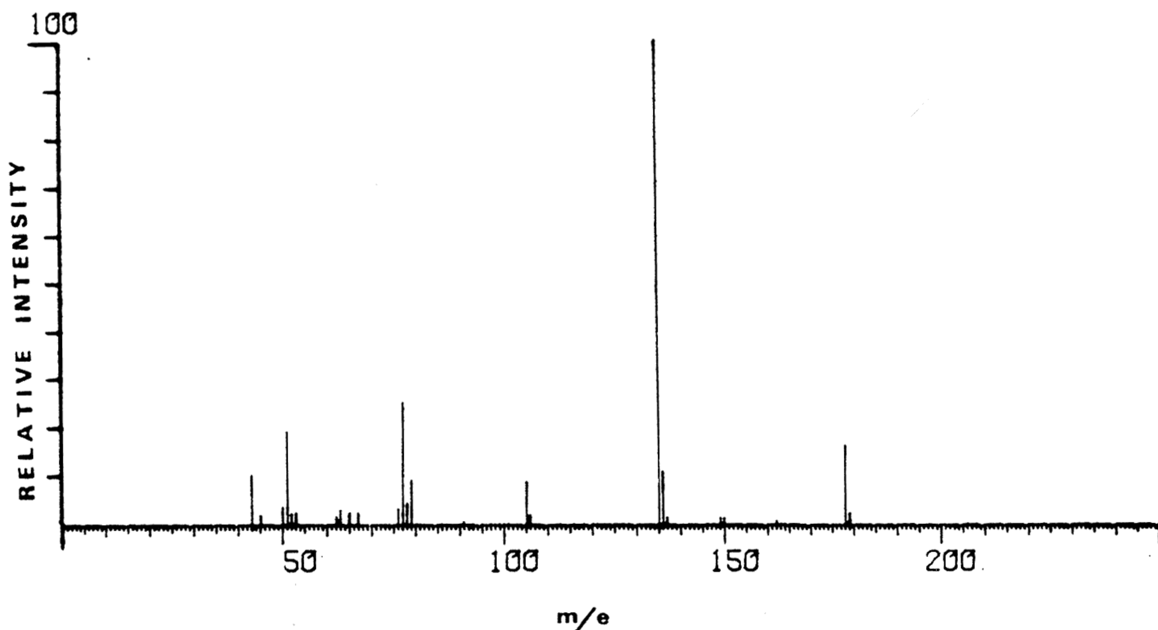
FIG. 8—Mass spectrum of 3,4-methylenedioxyphenyl-2-propanone.
