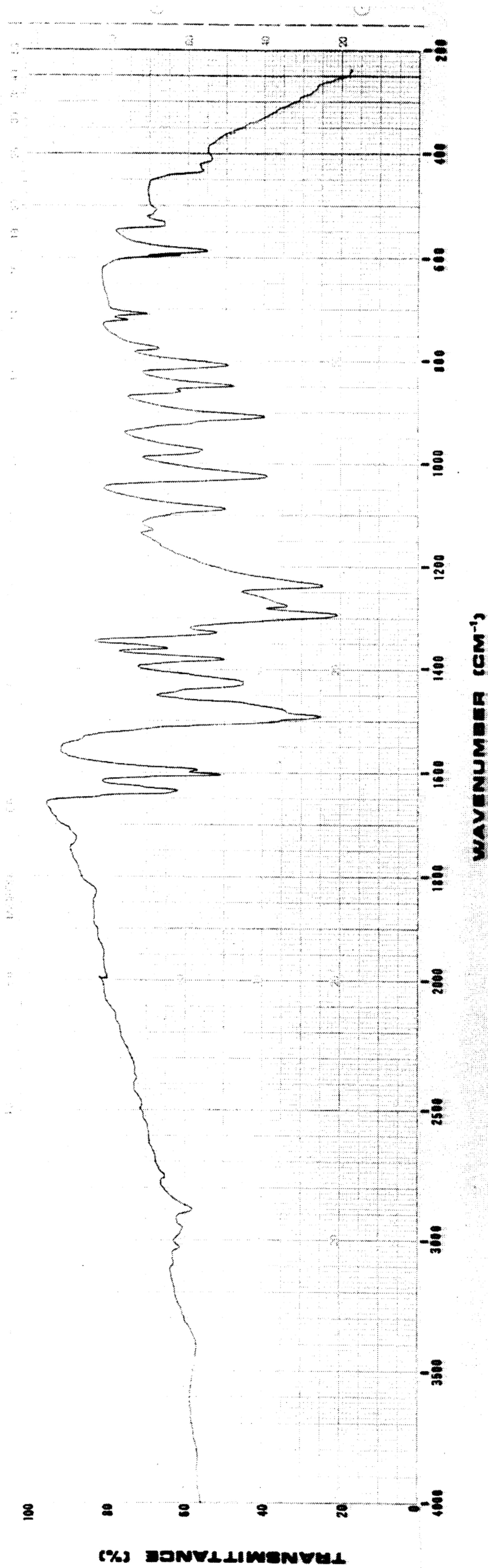
FIG. 16—IR spectra of A, piperonal and B, 1-(3,4-methylenedioxyphenyl)-2-nitro-1-propene.
