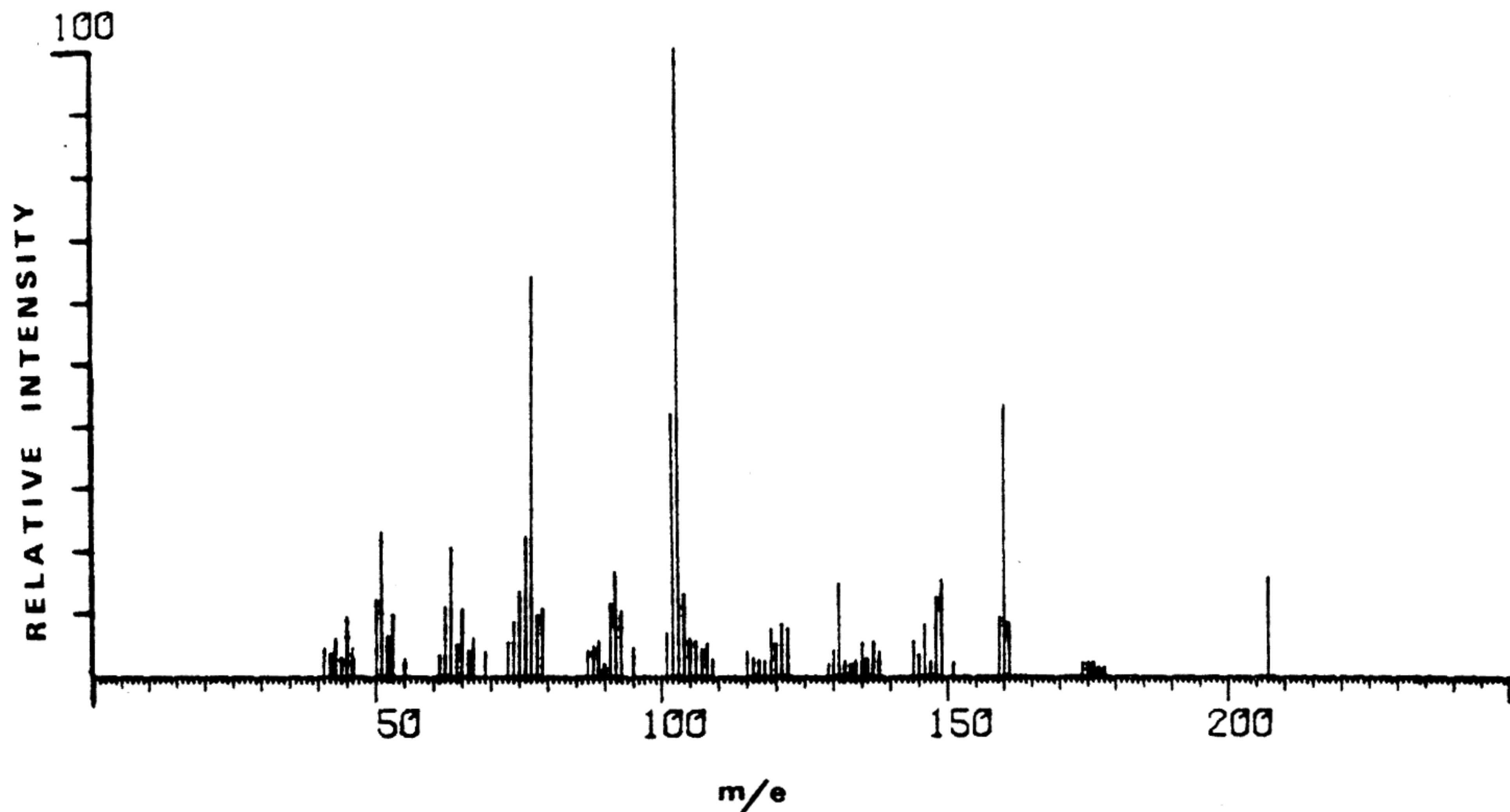
FIG. 17—Mass spectra of piperonal (top) and 1-(3,4-methylenedioxyphenyl)-2-nitro-1-propene (bottom).
