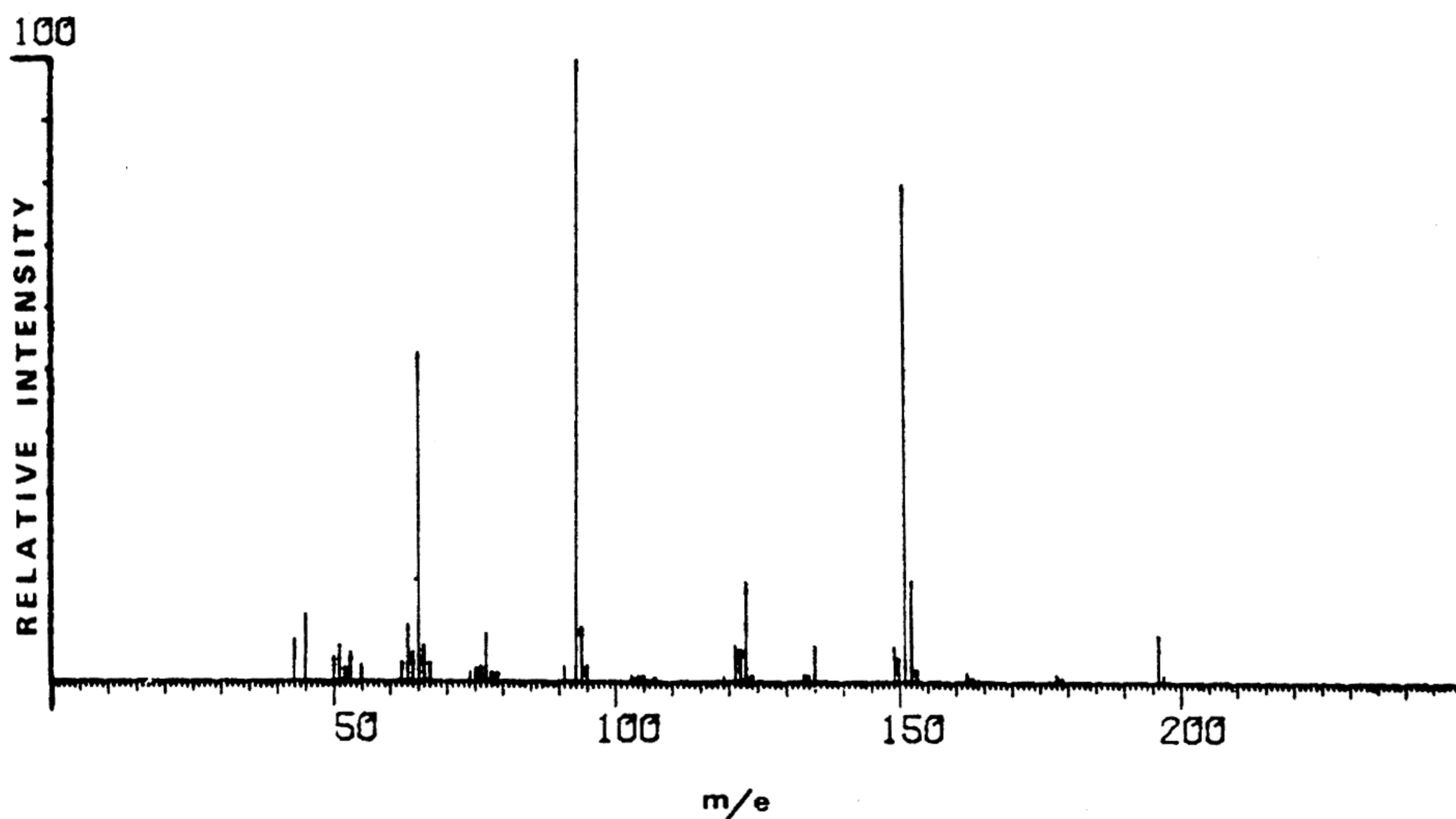
FIG. 6—Mass spectrum of isosafrole glycol.
