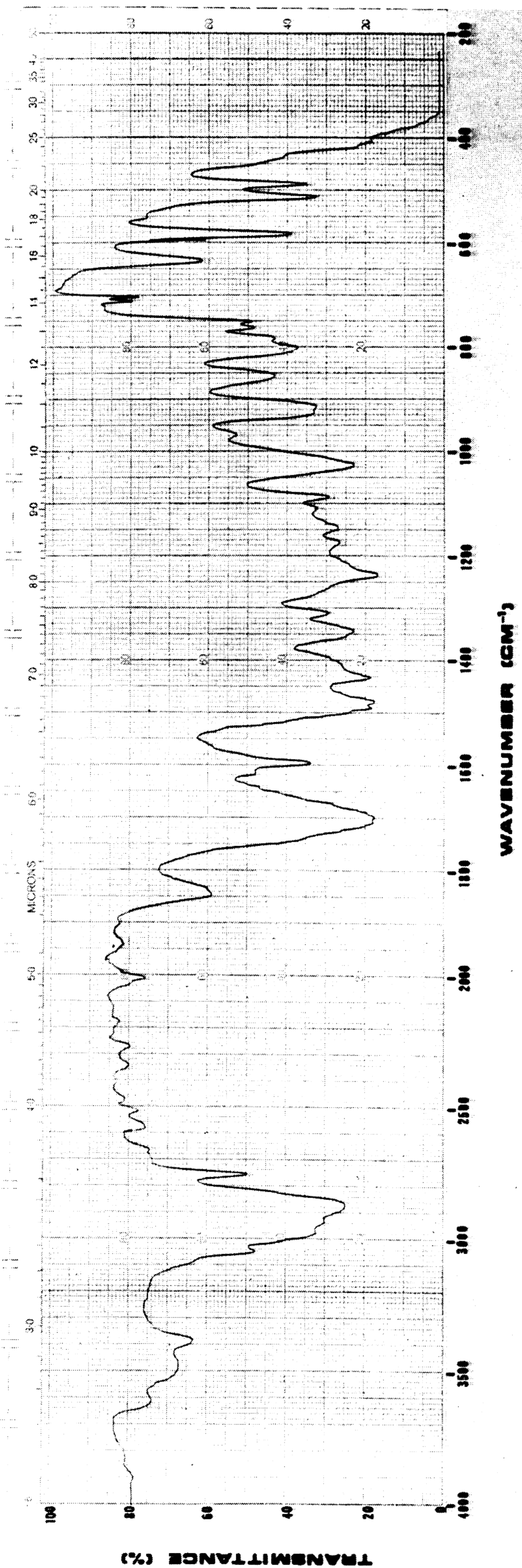
FIG. 7—IR spectrum of 3,4-methylenedioxyphenyl-2-propanone.
