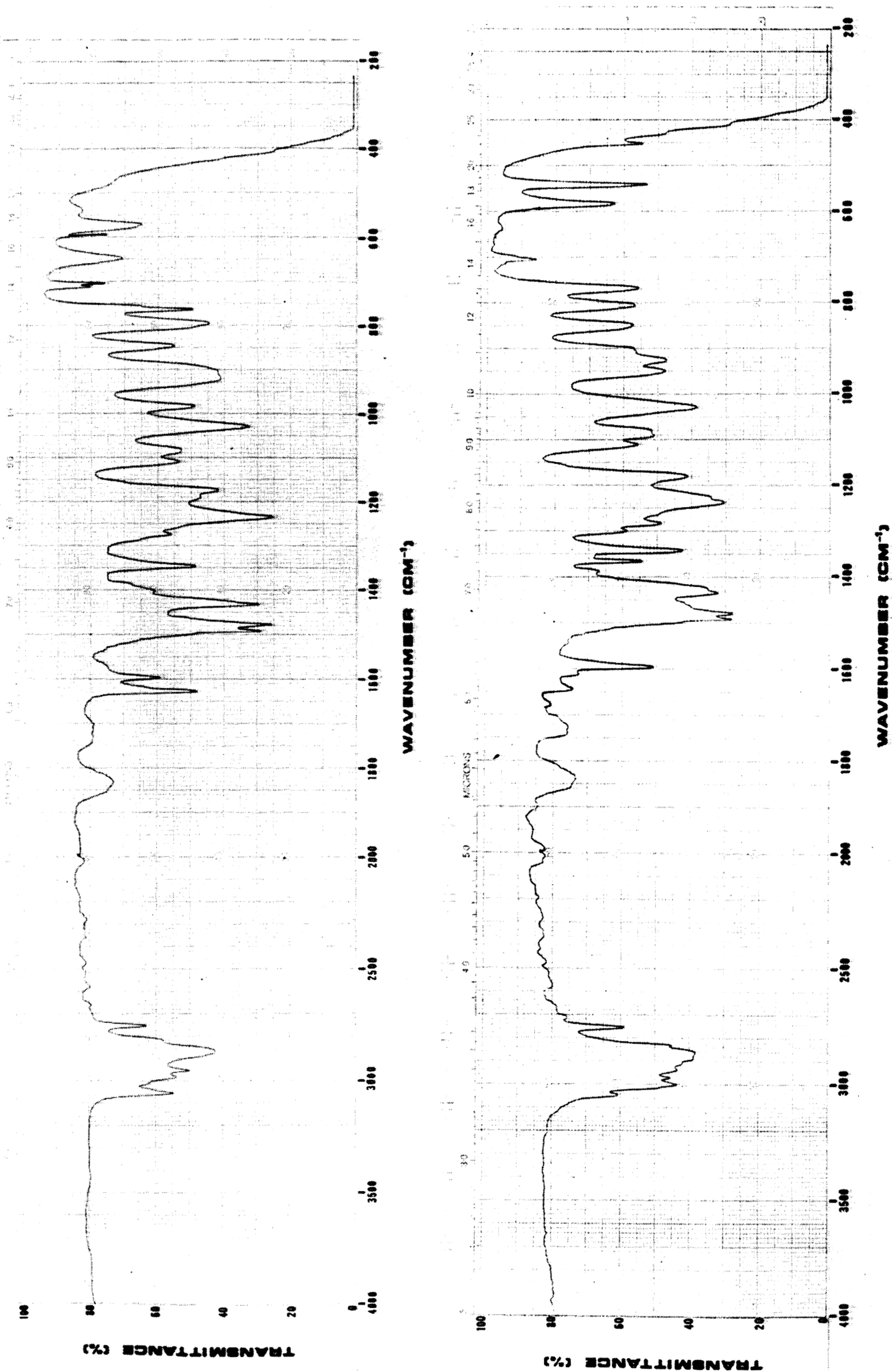
FIG. 3—IR spectra of safrole (top) and isosafrole (bottom).
