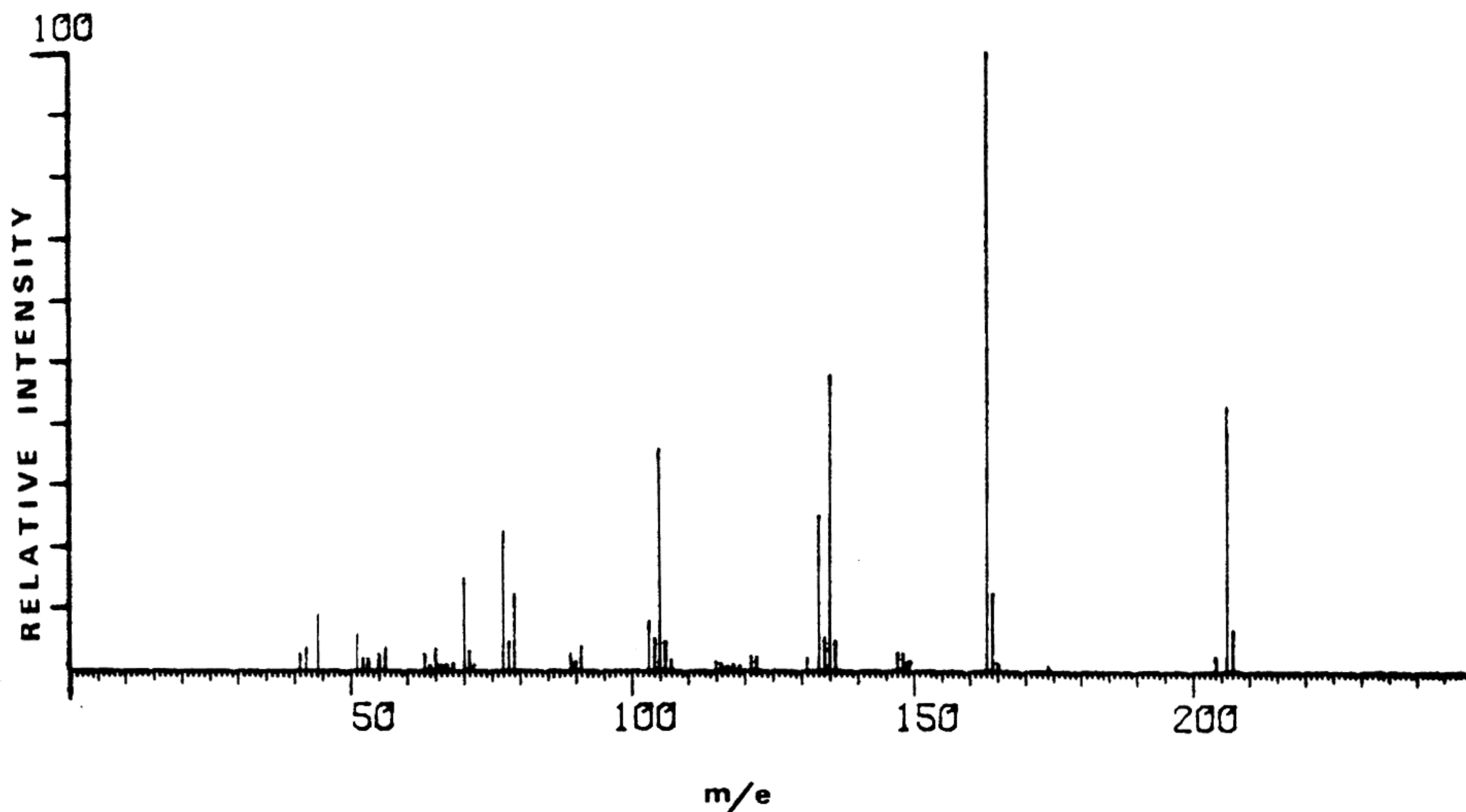
FIG. 15—Mass spectra of di[1-(3,4-methylenedioxyphenyl)-2-propyl]methylamine (top) and di[1-(3,4-methylenedioxyphenyl)-2-propyl]amine (bottom).
