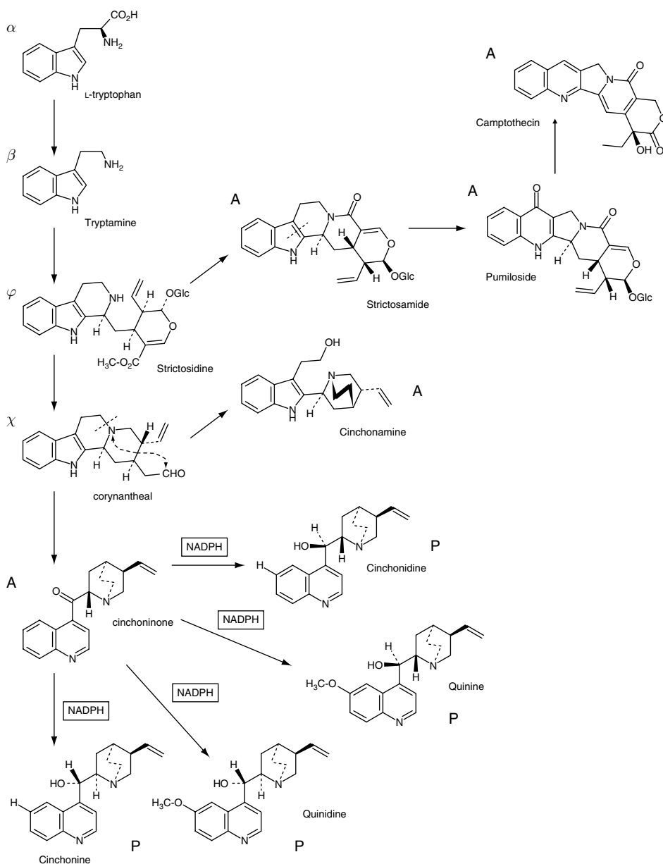
Figure 69. Structural development of quinoline alkaloids.
