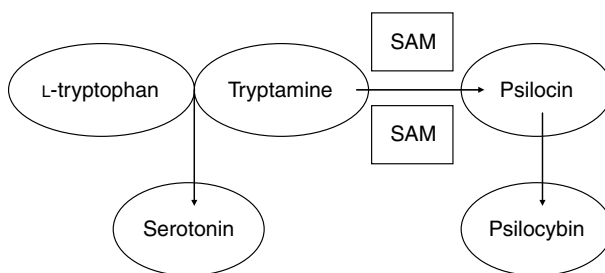
Figure 39. Psilocybin and serotonin synthesis pathway.
