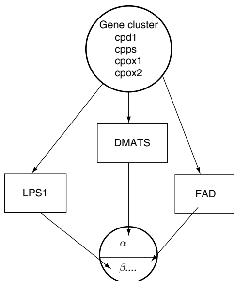
Figure 76. Molecular biology model of Claviceps purpurea alkaloids.
