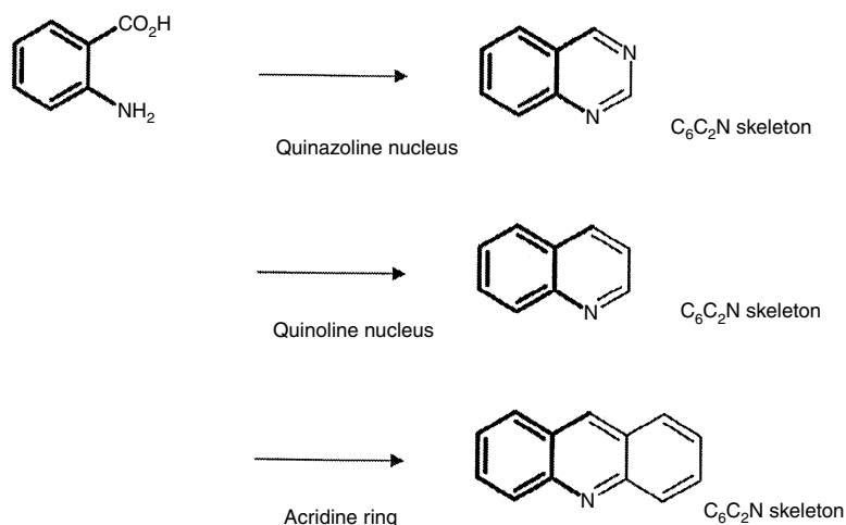
Figure 28. The nuclei produced by anthranilic acid in alkaloids.
