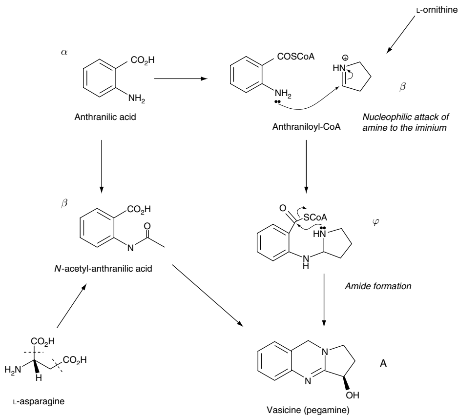
Figure 59. Structural development of quinazoline alkaloid vasicine.
