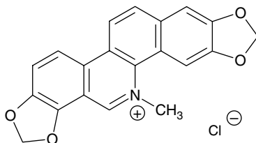
Figure 93. Sanguinarine, an alkaloid from Sanguinaria canadensis .
