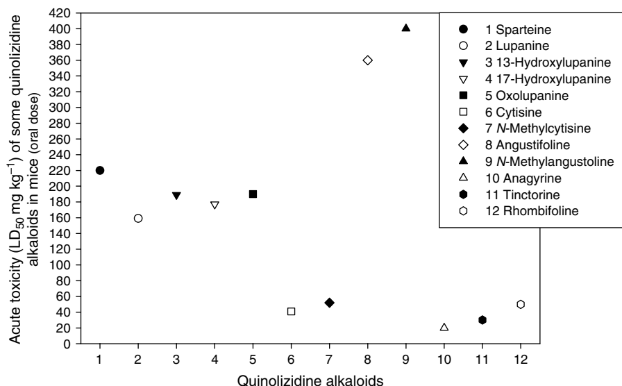
Figure 88. Acute toxicity (LD 50 ) of some quinolizidine alkaloids in mice (Refs [394, 472, 473, 474, 475]).
