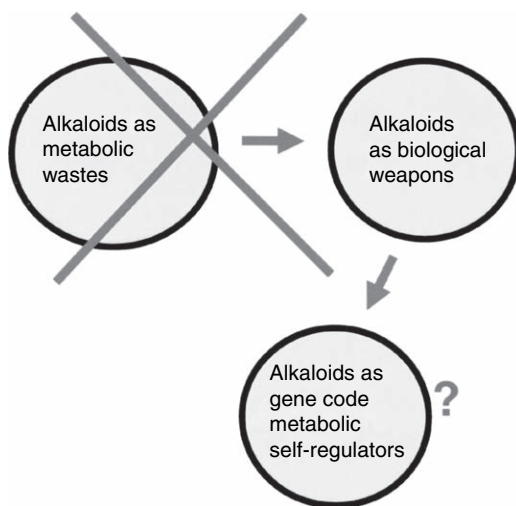
Figure 77. Three basic hypotheses on the biological nature of alkaloids.
