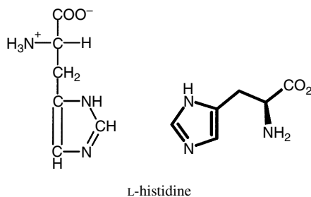
Figure 14. L-histidine is a precursor of imidazole alkaloids.
