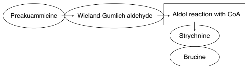
Figure 43. Diagram of the strychnine and brucine pathway.
