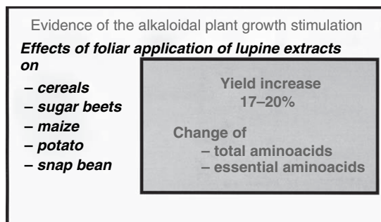
Figure 79. Effects of foliar application of lupine extracts.
