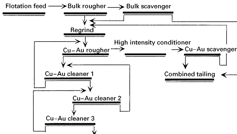
Figure 4 Bulk flow sheet used in the treatment of pyritic copper-gold ores. Reproduced with permission from Bulatovic (1997).
