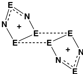
Fig. 4.9 Structure of E_6N_4^{2+} (E = S, Se)
