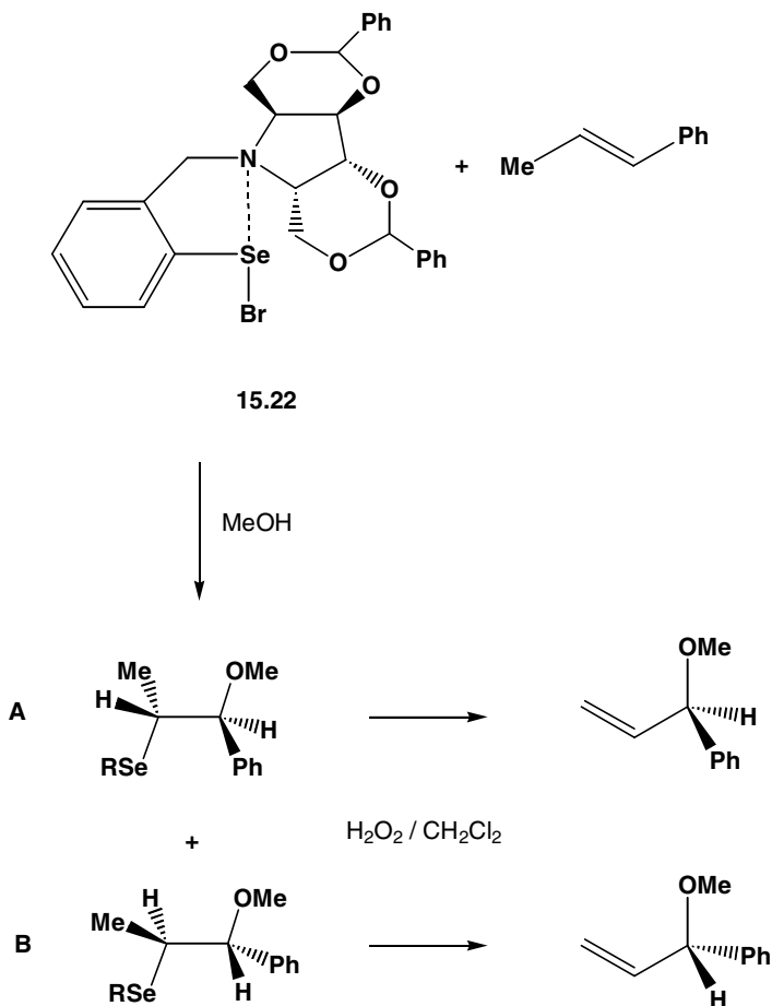
Scheme 15.2 Stereoselective control under the influence of an Se...N interaction
