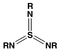
8.5a (R = SiMe 3 )
