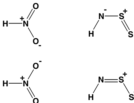
Scheme 10.3 Resonance structures for \text{HNO}_2 and \text{HNS}_2
