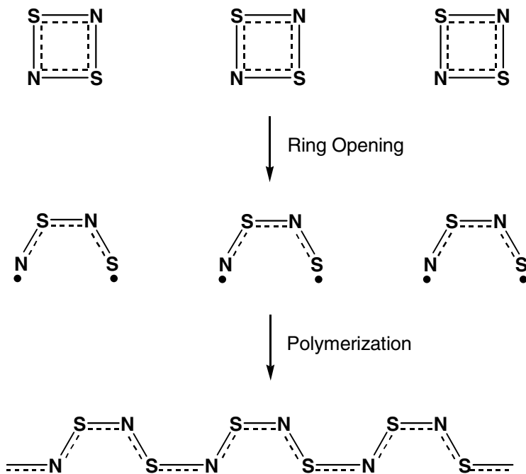
Fig. 14.1 Synthesis and structure of (\text{SN})_x
