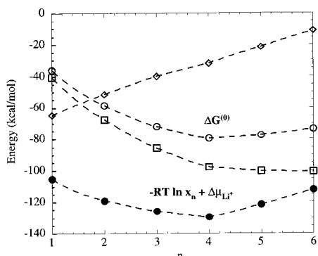
Figure 1. Free energies for \text{Li}^+ ion hydration in liquid water as a function of the number of inner shell water neighbors at T = 298.15 K. The results marked \Delta G^{(0)} (open circles) are the free energies predicted for the reaction \text{Li}^+ + n\text{H}_2\text{O} \rightleftharpoons \text{Li}(\text{H}_2\text{O})_n^+ under standard ideal conditions, including p = 1 atm. The minimum value is at n = 4 . The next lower curve (squares) incorporates the replacement free energy -RT \ln(RT \rho_w/1 \text{ atm}) that adjusts the concentration of water molecules to the normal concentration of liquid water, \rho_w = 1 \text{ g/cm}^3 so that RT\rho_w = 1354 \text{ atm} . 35 The minimum value is at n = 6 . The topmost graph (diamonds) plots \mu_{\text{Li}(\text{H}_2\text{O})_n^*} - n\mu_{\text{H}_2\text{O}}^* , the external-cluster contributions obtained from the standard dielectric model. 34,35 The bottommost results (solid circles) are the final, net values. The label provides the quasi-chemical interpretation of these net values 33,36 with x_n the fraction of lithium ions having n inner shell water neighbors and \Delta\mu_{\text{Li}^+} the interaction part of the chemical potential of the lithium ions. This graph indicates that the n = 4 inner sphere structure is most probable in liquid water under normal conditions.
