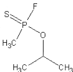
Thiosarin
