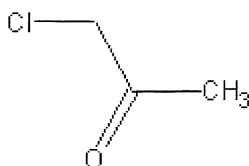
Chloroacetone
