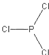
Phosphorus trichloride
