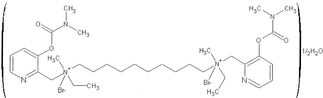
Chemical agent 4-686-293-01
