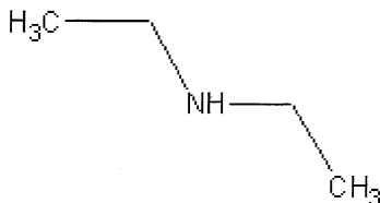
Diethylamine
