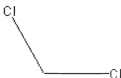
Methylene chloride
