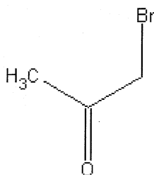
Bromoacetone
