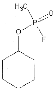
Cyclosarin
