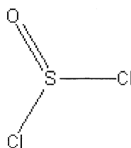
Thionyl chloride
