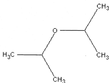
Isopropyl ether
