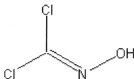
Phosgene oxime
