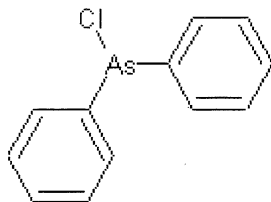
Diphenylchloroarsine
