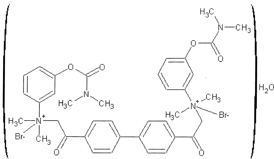
Chemical agent 4-692-530-02
