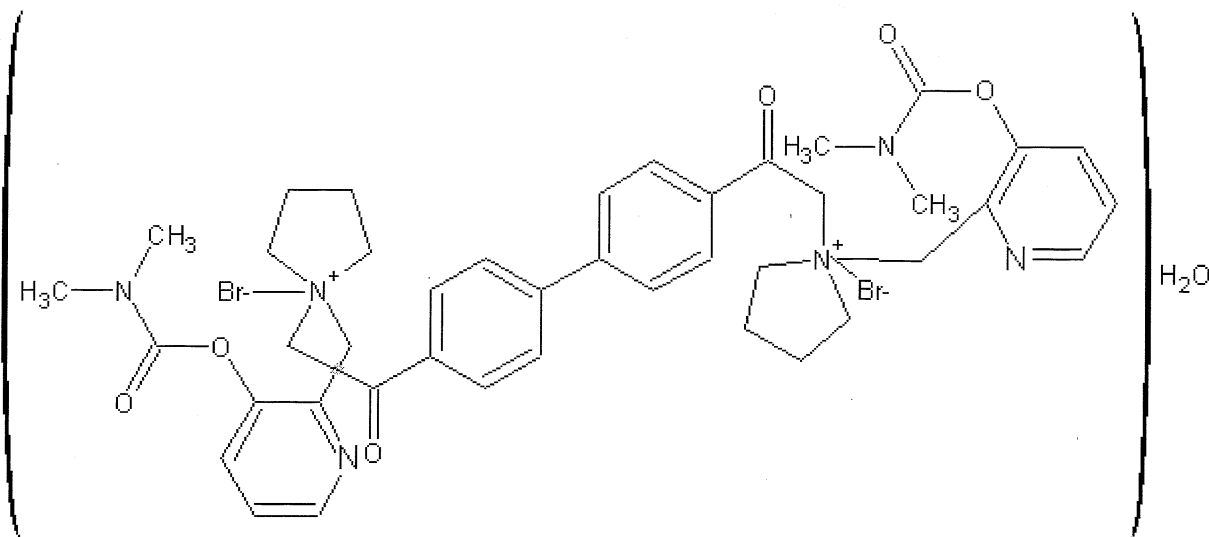
Chemical agent 4-692-530-01
