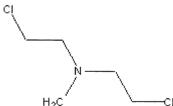
HN2
