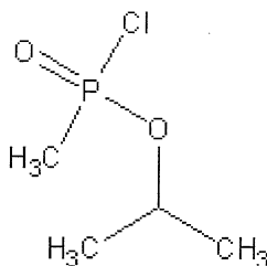
Chlorosarin
