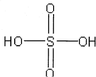
Sulfuric acid
