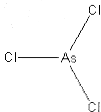
Arsenic trichloride
