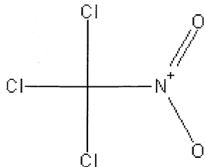
Chloropicrin
