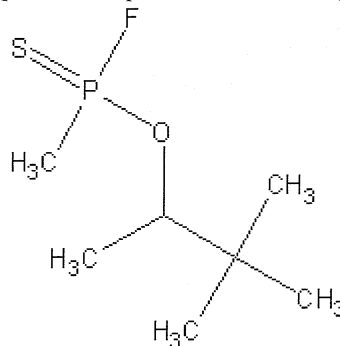
Thiosoman
