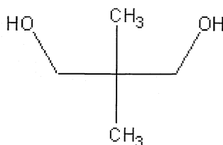
Neopentyl glycol
