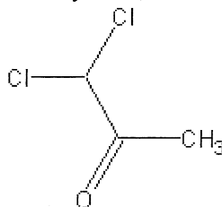
Dichloroacetone
