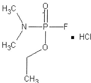
FluoroTabun Hydrochloride
