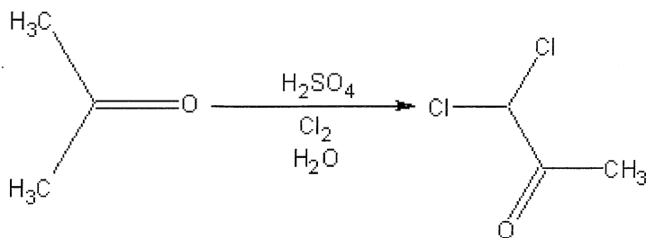
Dichloroacetone
