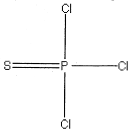
Thiophosphorus trichloride
