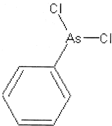
Phenyldichloroarsine
