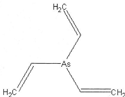
VS
