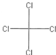
Carbon tetrachloride
