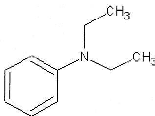
Diethylaniline
