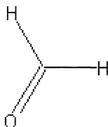
Formaldehyde
