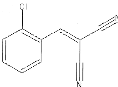
CS
