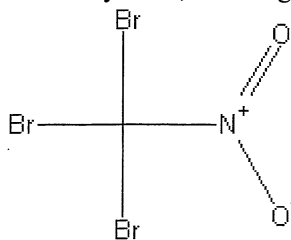
Bromopicrin
