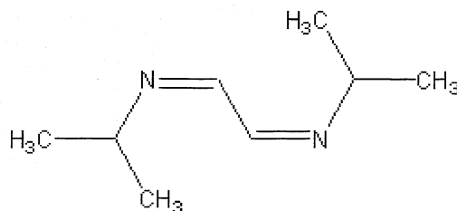
DIIMINE
