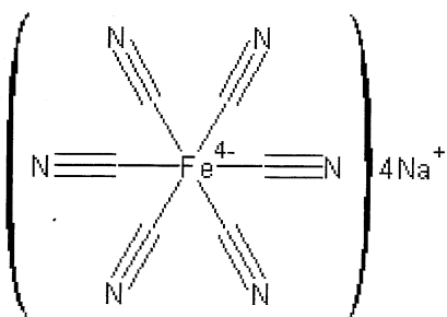
Sodium ferrocyanide
