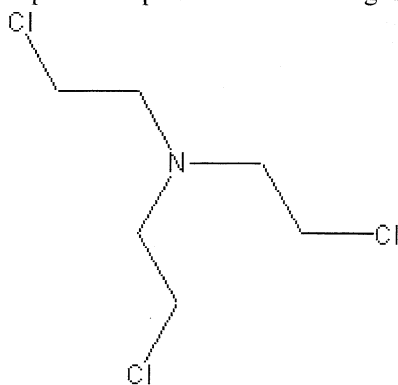
HN3
