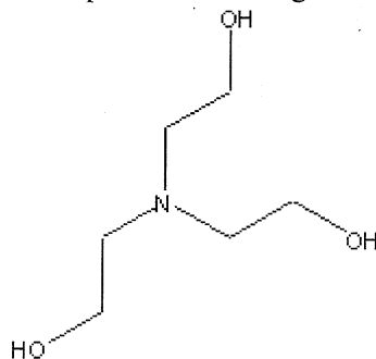
Triethanolamine
