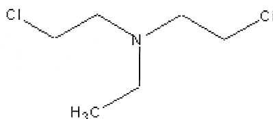
HN1
