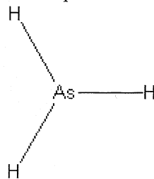
Arsine
