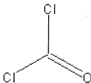
Phosgene
