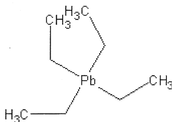
Tetraethyl lead
