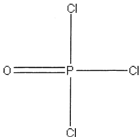
Phosphorus oxychloride
