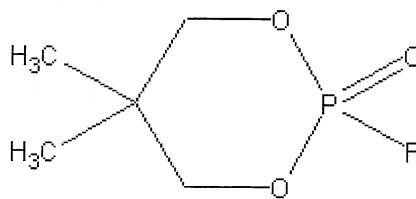
NPF
