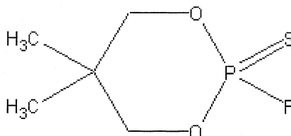
NPSF
