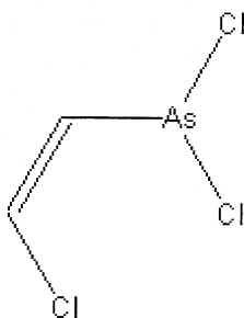
Lewisite
