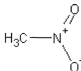
Nitromethane
