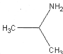
Isopropylamine
