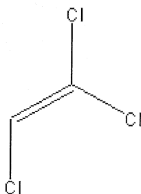
Trichloroethylene
