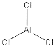
Aluminum chloride
