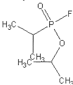
Sarin-isopropyl
