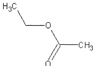
Ethyl acetate
