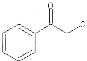
CN
