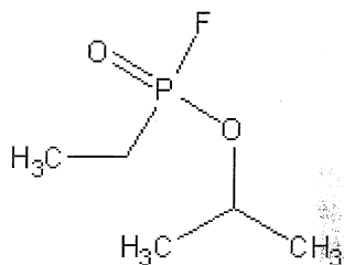
Sarin-Ethyl
