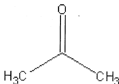
Acetone
