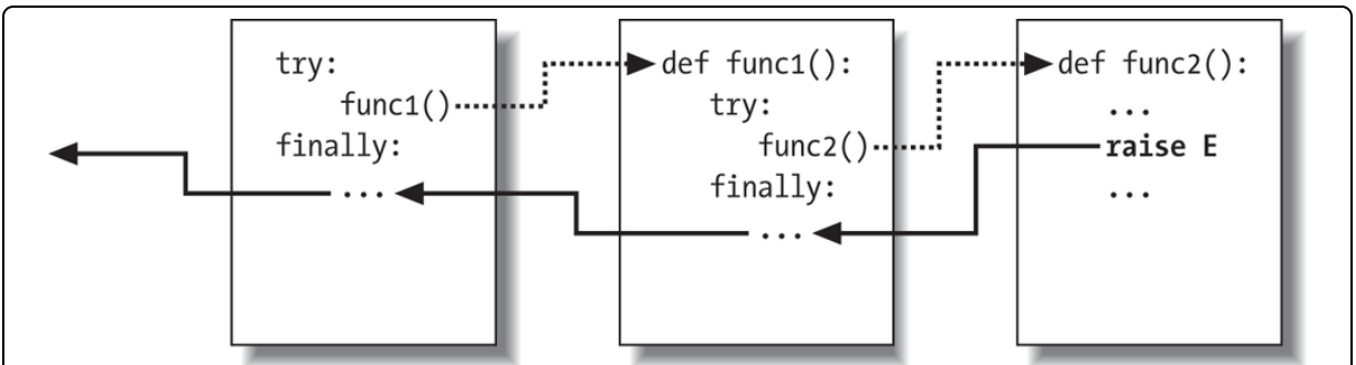
Figure 36-2. Nested try/finally statements: when an exception is raised, control returns to the most recently entered try to run its finally statement, but then the exception keeps propagating to all finallys in all active try statements and eventually reaches the default top-level handler where an error message is printed. finally clauses do not (but do not stop) an exception—they are for actions to be performed “on the way out.”
