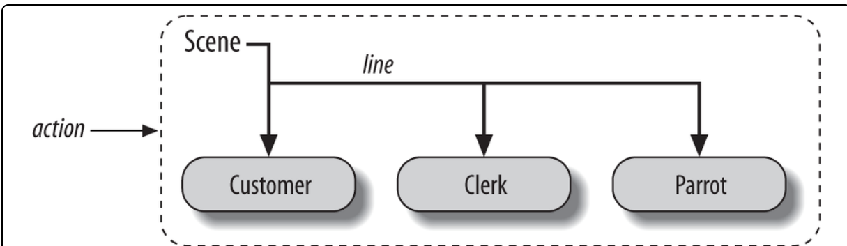
Figure 32-2. A scene composite with a container class ( Scene ) that embeds and delegates instances of the other classes ( Customer , Clerk , Parrot ). The embedded instance classes may all so participate in an inheritance hierarchy; composition and inheritance are often equally useful ways to structure classes for code reuse.
