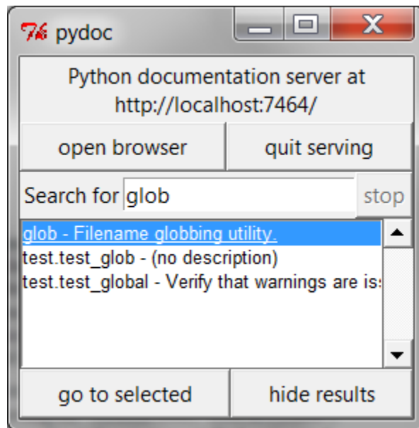
Figure 15-3. The PyDoc top-level search engine GUI client in 3.2 and earlier: type the name of the module you want documentation for, press Enter, select the module, and then press “go to selected” (or omit the module name and press “open browser” to see all available modules).
