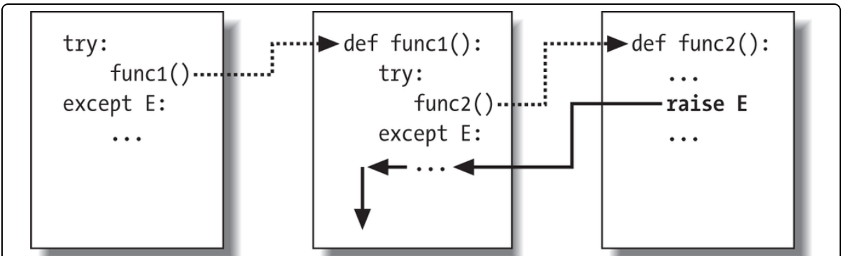
Figure 36-1. Nested try/except statements: when an exception is raised (by you or by Python), control jumps back to the most recently entered try statement with a matching except clause, and the program resumes after that try statement. except clauses intercept and stop the exception—they are where you process and recover from exceptions.
