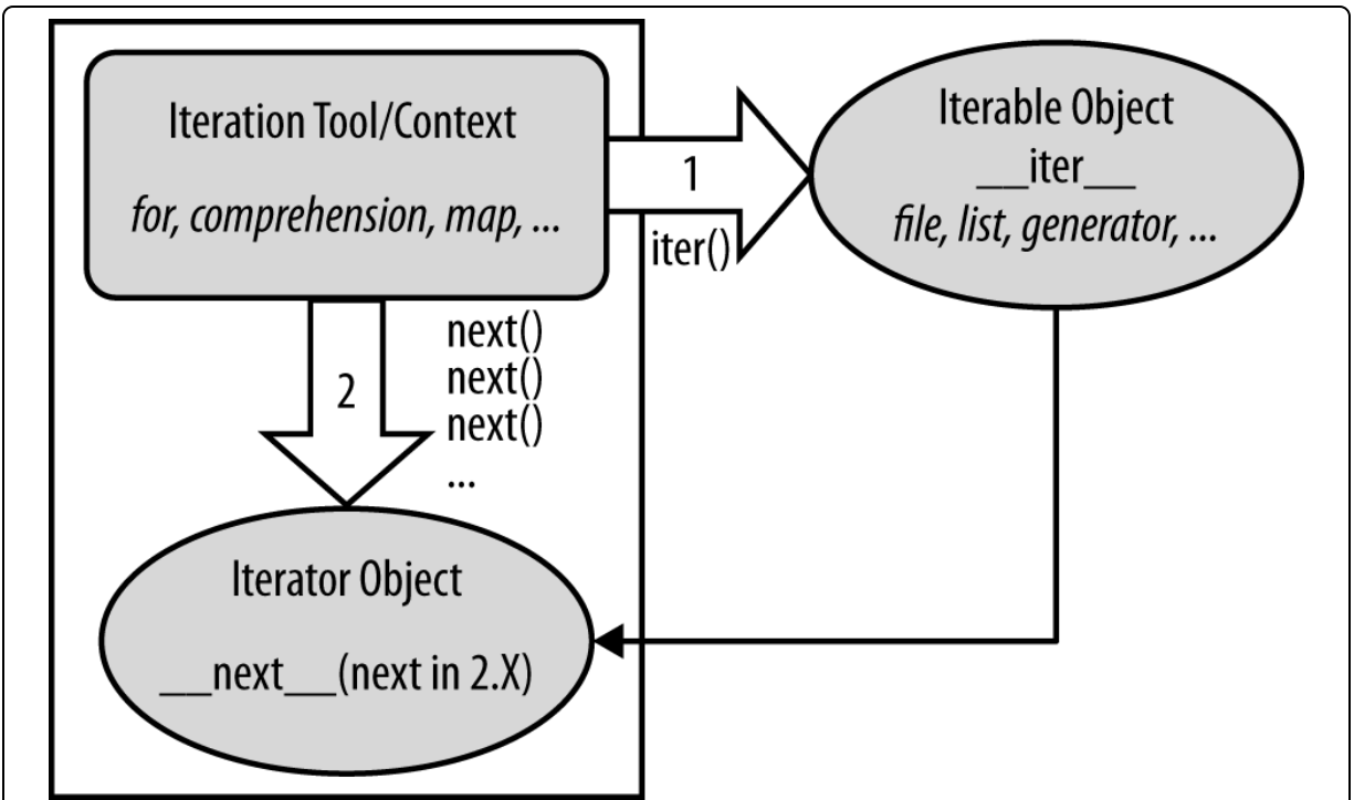
Figure 14-1. The Python iteration protocol, used by for loops, comprehensions, maps, and more, and supported by files, lists, dictionaries, Chapter 20's generators, and more. Some objects are both iteration context and iterable object, such as generator expressions and 3.X flavors of some tools (such as map and zip). Some objects are both iterable and iterator, returning themselves for the iter() call, which is then a no-op.
