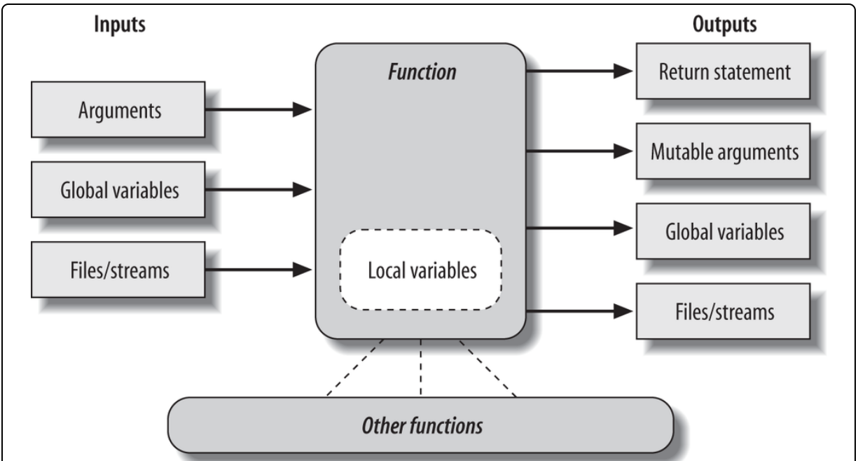
Figure 19-1. Function execution environment. Functions may obtain input and produce output in a variety of ways, though functions are usually easier to understand and maintain if you use arguments for input and return statements and anticipated mutable argument changes for output. In Python 3, outputs may also take the form of declared local names that exist in an enclosing function scope.
