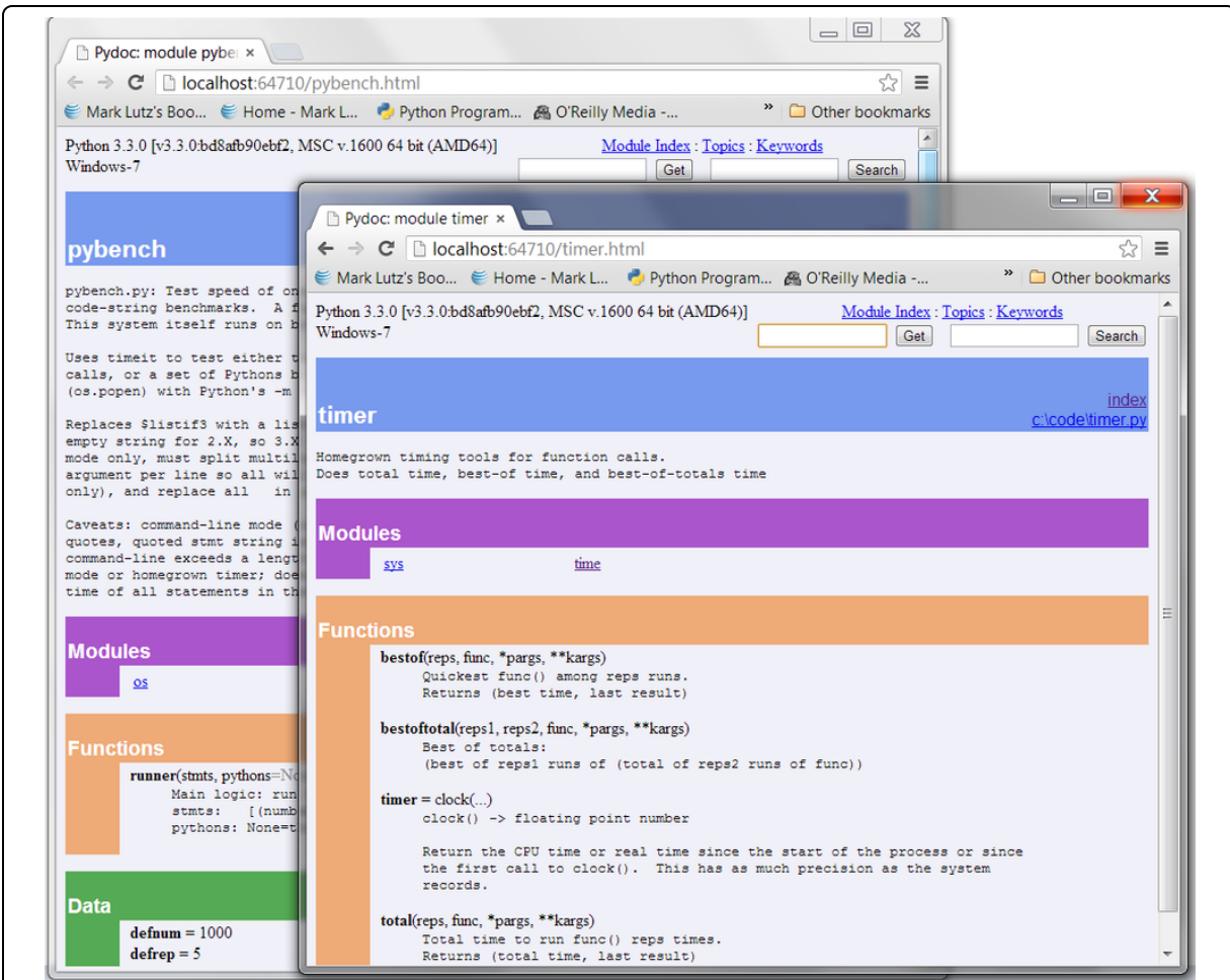
Figure 15-2. PyDoc's module display page in Python 3.2 and later with input fields at the top. To display two modules we will be coding in the next part of this book (Chapter 21).
