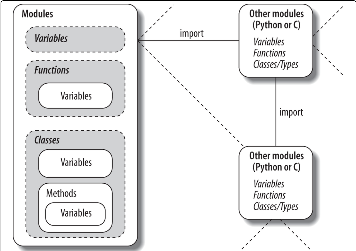
Figure 25-1. Module execution environment. Modules are imported, but modules also import and use other modules, which may be coded in Python or another language such as C. Modules in turn contain variables, functions, and classes to do their work, and their functions and classes may contain variables and other items of their own. At the top, though, programs are just sets of modules.
