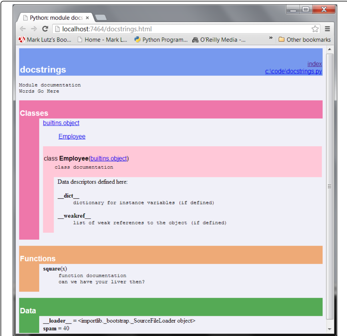
Figure 15-5. PyDoc can serve up documentation pages for both built-in and user-defined modules on the module search path. Here is the page for a user-defined module, showing all its documentation strings (docstrings) extracted from the source file.
