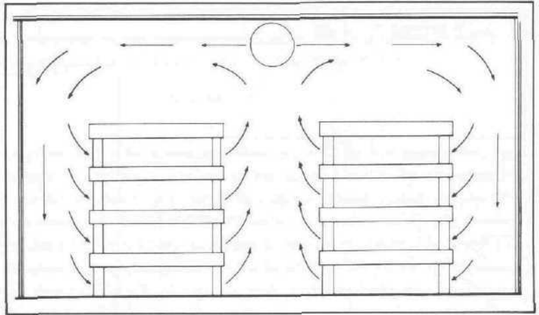
Figure 74 Central aisle outward flow air circulation pattern.
