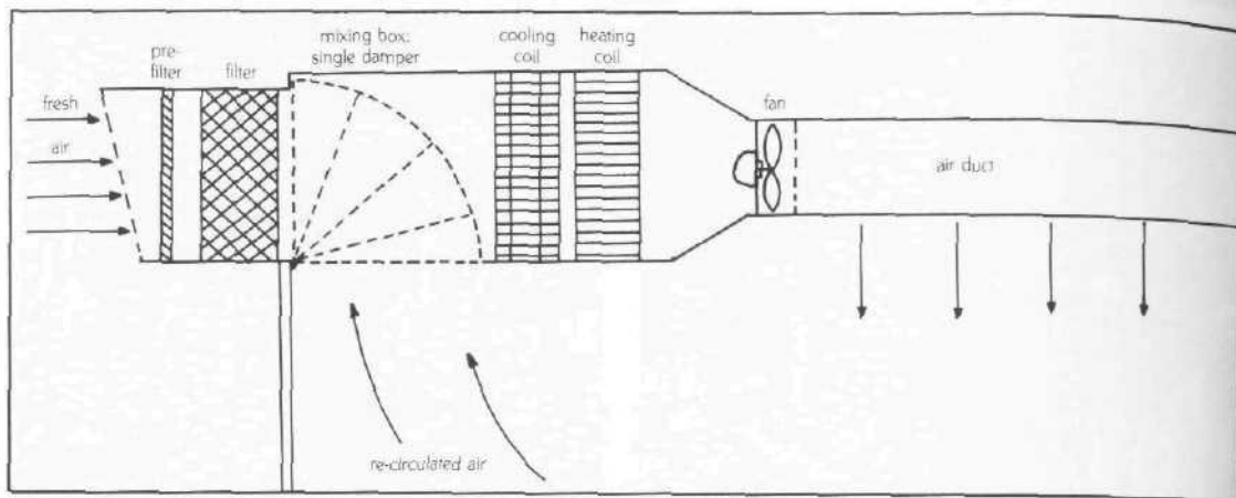
Figure 73 Standard ventilation system used by Agaricus growers. (After Vedder)
