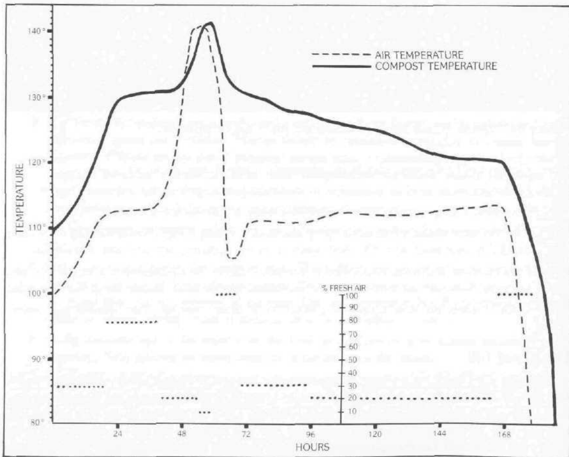
Figure 97 Phase II temperature profile for trays or shelves.
