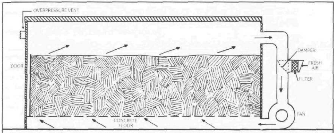
Figure 98 Bulk pasteurization room. Ventilation system on end wall. (Design—Vedder)
