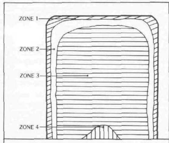
Figure 89 Temperature zonation during Short Composting.
