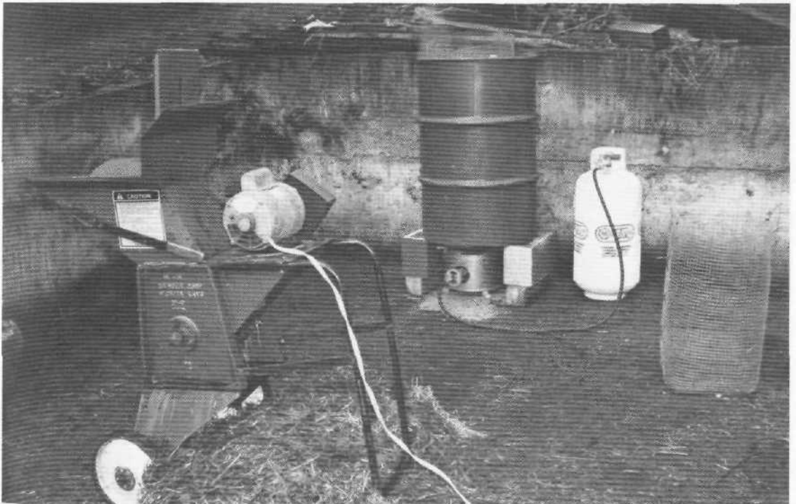
Figure 111 Equipment needed for pasteurization of straw: 55 gallon drum; gas burner; shredder; hardware cloth basket and straw.
