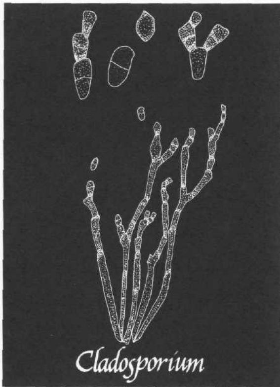
Figure 195 Drawing of Cladosporium . Note the two celled conidia.
