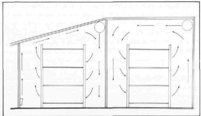
Figure 76 Wall mounted duct directing airflow across the width or down the sidewall of the room.
