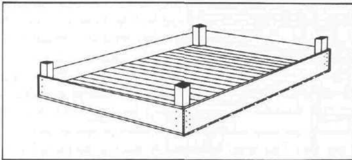
Figure 68 Sinden system tray. The tray can be constructed of 1 x 6 or 2 x 6 inch lumber for bottom and side boards and 4 x 4 inch corner posts. (1 x 8 or 2 x 8 inch side boards are suggested for deep fills).
