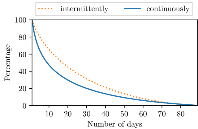
Figure 7: Percentage of peers that we see in the network continuously or intermittently for n days.
