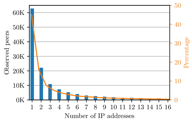
Figure 8: Number of IP addresses I2P peers are associated with.
